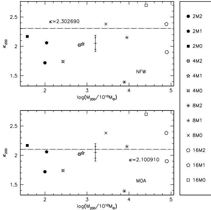
Fig. 4. Deviation of simulated dark matter haloes from their fitting counterparts, with respect to the dimensionless parameter \kappa_{200} , for both NFW (top) and MOA (bottom) self-similar, universal density profiles. Other captions as in Fig. 1.
