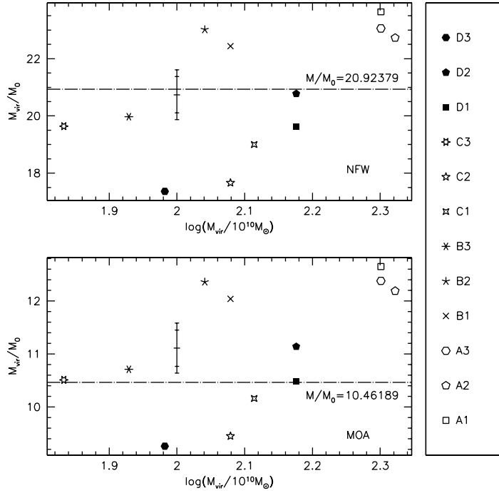
Fig. 5. Deviation of simulated dark matter haloes from their fitting counterparts, with respect to the scaled virial mass M_{\text{vir}}/M_0 , for both NFW (top) and MOA (bottom) self-similar, universal density profiles. Fitting haloes lie on the horizontal line, while simulated haloes are represented by different symbols. The vertical bar is centred on the mean value of plotted data, with respect to the ordinates (and no connection with the abscissae), and is limited by the standard deviation of the mean, without (inner boundary) and with (outer boundary) addition of about twice the standard deviation from the standard deviation from the mean, deduced from Eqs. (23), (24), and (25), respectively. Captions of symbols on the right correspond to KLA01 runs listed in Tables 4, 6, and 8.
