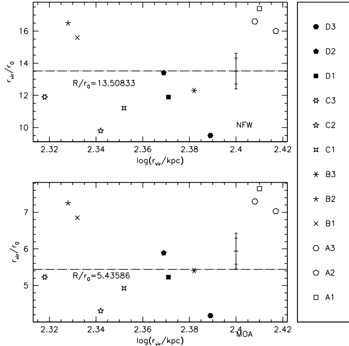
Fig. 6. Deviation of simulated dark matter haloes from their fitting counterparts, with respect to the scaled radius r_{\text{vir}}/r_0 , for both NFW (top) and MOA (bottom) self-similar, universal density profiles. Other captions as in Fig. 5.
