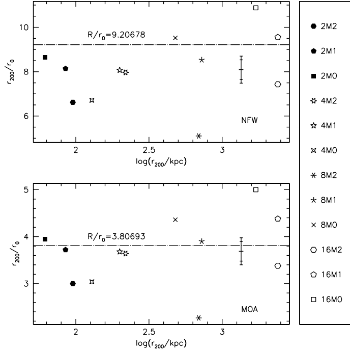
Fig. 2. Deviation of simulated dark matter haloes from their fitting counterparts, with respect to the scaled radius r_{200}/r_0 , for both NFW (top) and MOA (bottom) self-similar, universal density profiles. Other captions as in Fig. 1.
