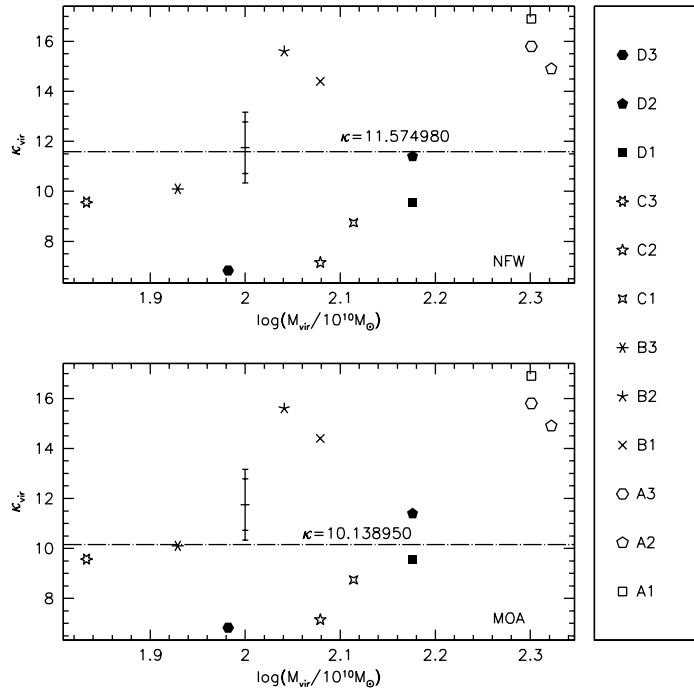
Fig. 8. Deviation of simulated dark matter haloes from their fitting counterparts, with regard to the dimensionless parameter \kappa_{vir} , for both NFW (top) and MOA (bottom) self-similar, universal density profiles. Other captions as in Fig. 5.
