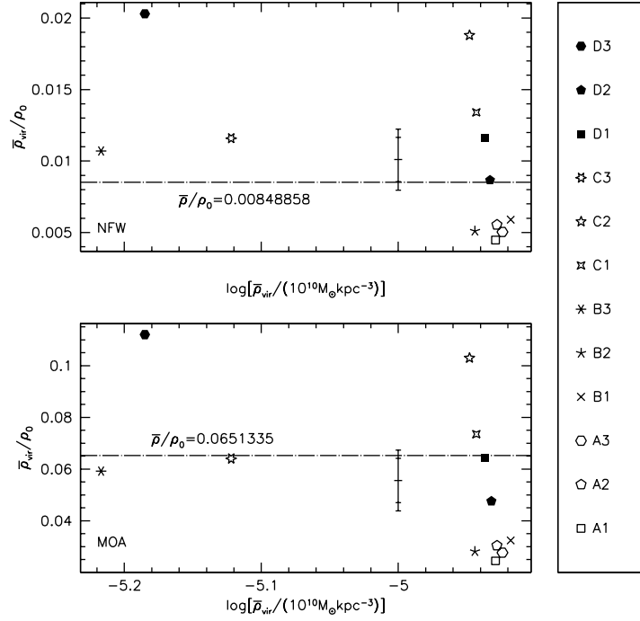
Fig. 7. Deviation of simulated dark matter haloes from their fitting counterparts, with respect to the scaled density \bar{\rho}_{vir}/\rho_0 , for both NFW (top) and MOA (bottom) self-similar, universal density profiles. Other captions as in Fig. 5.
