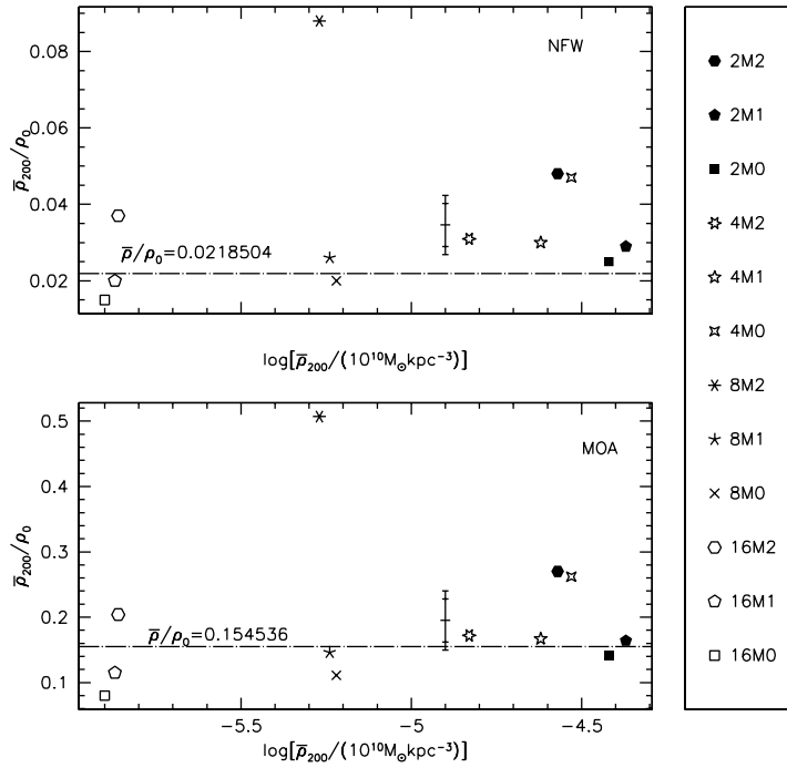
Fig. 3. Deviation of simulated dark matter haloes from their fitting counterparts, with respect to the scaled density \bar{\rho}_{200}/\rho_0 , for both NFW (top) and MOA (bottom) self-similar, universal density profiles. Other captions as in Fig. 1.
