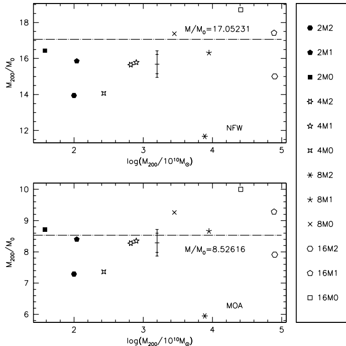
Fig. 1. Deviation of simulated dark matter haloes from their fitting counterparts, with respect to the scaled virial mass M_{200}/M_0 , for both NFW (top) and MOA (bottom) density profiles. Fitting haloes lie on the horizontal line, while simulated haloes are represented by different symbols. The vertical bar is centred on the mean value of plotted data, with respect to the ordinates (and no connection with the abscissae), and is limited by the standard deviation from the mean, without (inner boundary) and with (outer boundary) addition of about twice the standard deviation from the standard deviation from the mean, deduced from Eqs. (23), (24), and (25), respectively. Captions of symbols on the right correspond to FM01 runs listed in Tables 3, 5, and 7.
