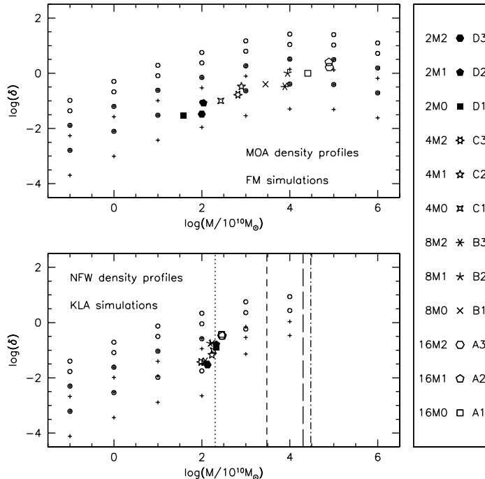
Fig. 9. The dimensionless parameter \delta vs. the fitting mass M for top-hat, spherical perturbations, with no (open circles) and maximum allowed (crosses) acquisition of angular momentum, according to Eqs. (40b) and (40c), in connection with MOA (top panel) and NFW (bottom panel) density profiles. For each mass and class of symbols, values from down to up are related to mean peak heights at recombination epoch, \bar{\nu}_{\text{rec}} = 1, 2, 3, 4 , respectively. The mass of the critical density perturbation, for which the turnaround radius is infinite, is marked by a vertical line, from the left to the right for increasing peak height (bottom panel). Values related to FM01 (top panel) and KLA01 (bottom panel) simulations are also represented, with same symbol captions as in Figs. 1-4 and 5-8, respectively. Passing from NFW to MOA density profile, for each set of simulations, would lower values related to top-hat, spherical perturbations by about one dex, and vice versa.
